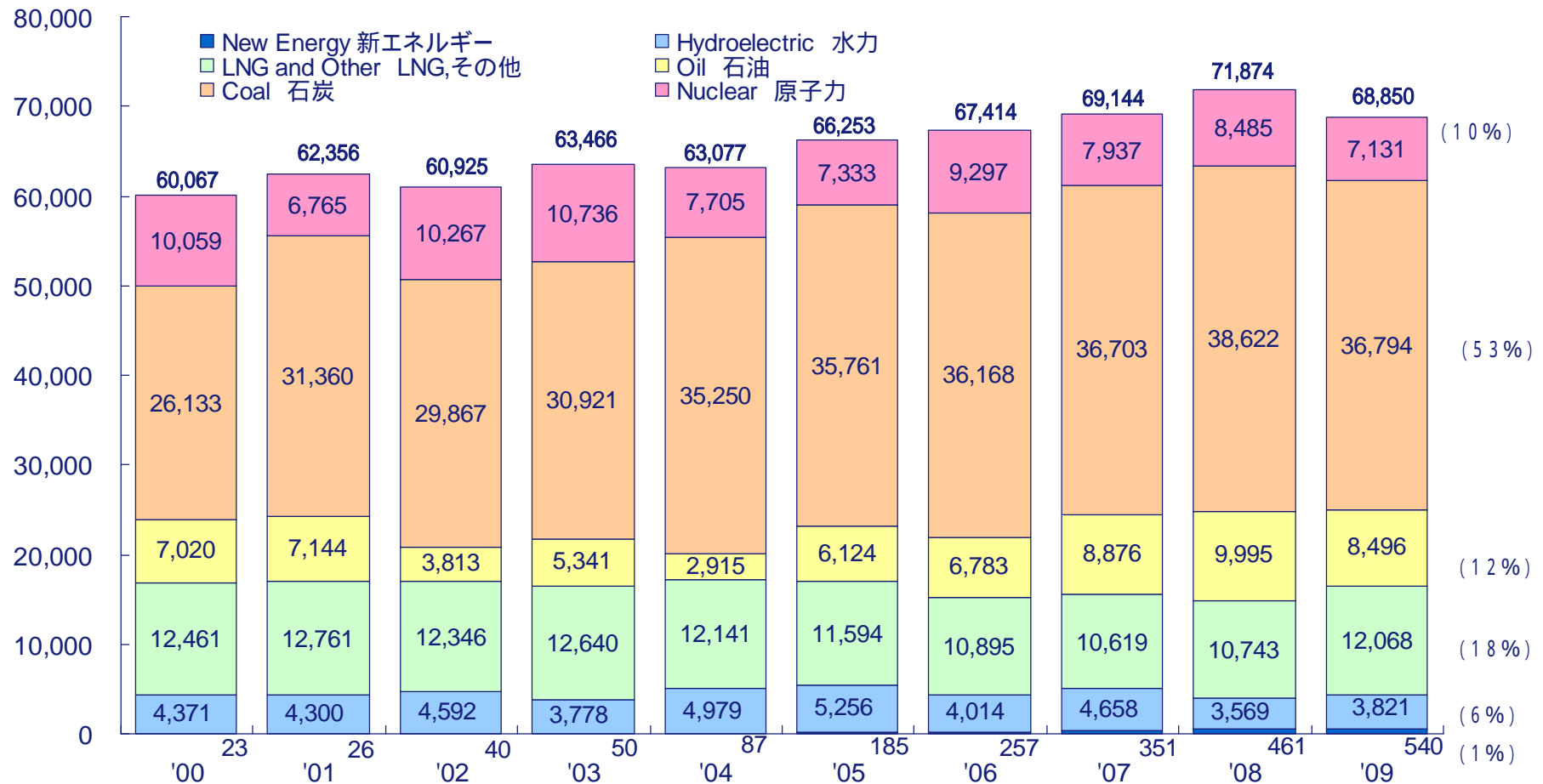
The Power Generation by Type 電源種別発電電力量 (Millions of kWh/100万kWh)
